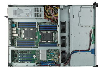
Optional 3*full-height expansion cards version
