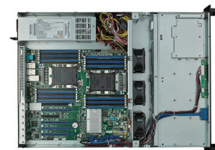
Standard 7*low-profile expansion cards version
